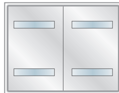
suspended ceiling 2-sectional, light area 4x 150 x 850 mm with LED-light panel
