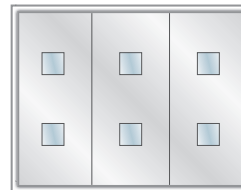
suspended ceiling 3-sectional, light area 6x 250 x 250 mm with LED-light panel
